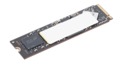
ThinkPad 1TB Performance PCIe Gen4 NVMe OPAL2 M.2 2280 SSD IV
